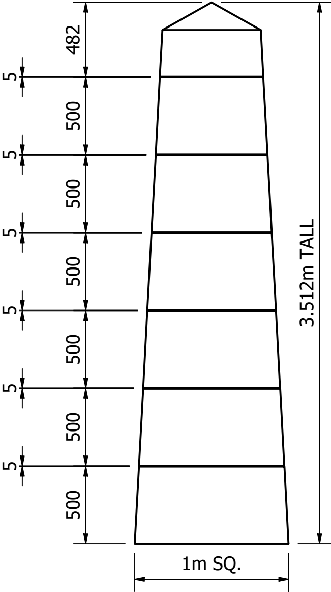
Jointing Heights ( 1 : 25 )
